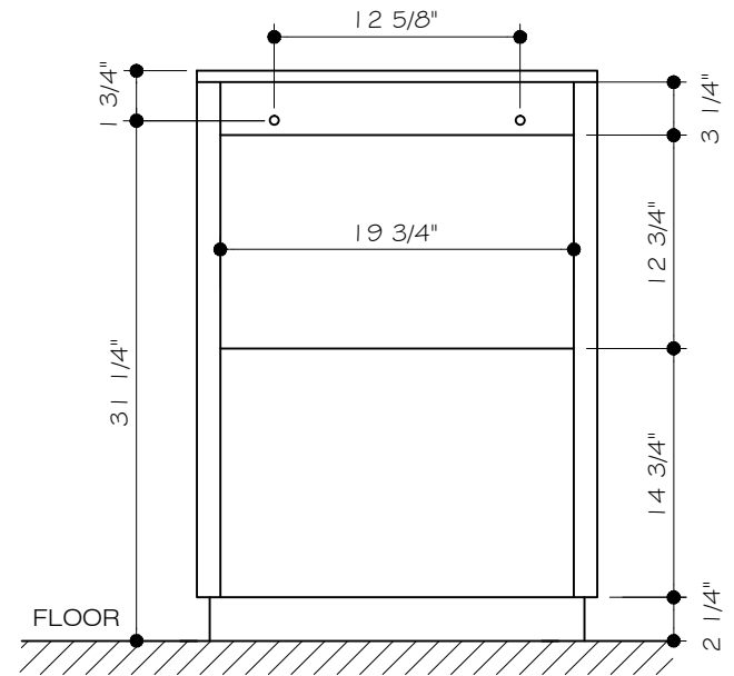
BACK VIEW
