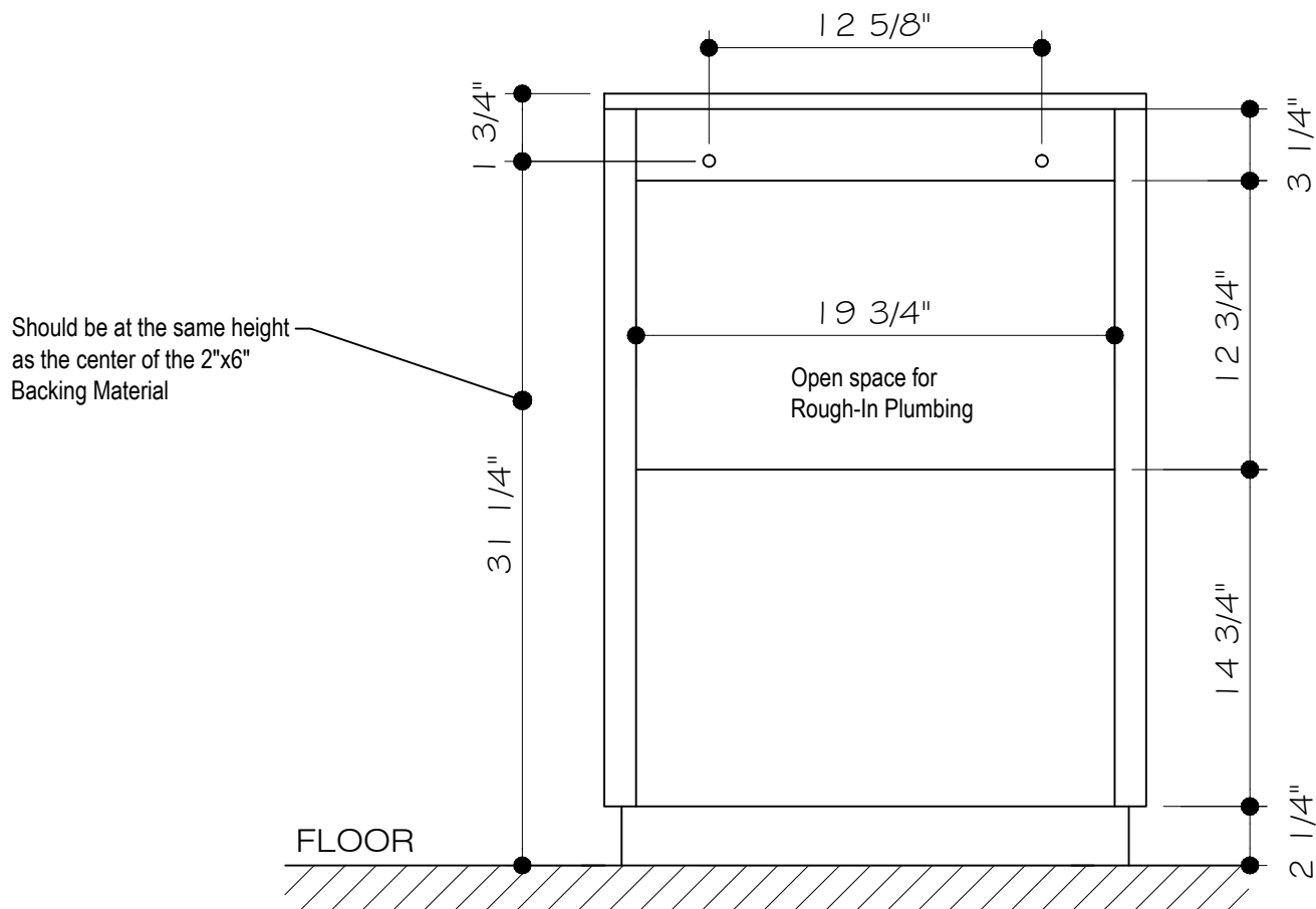
BACK VIEW
