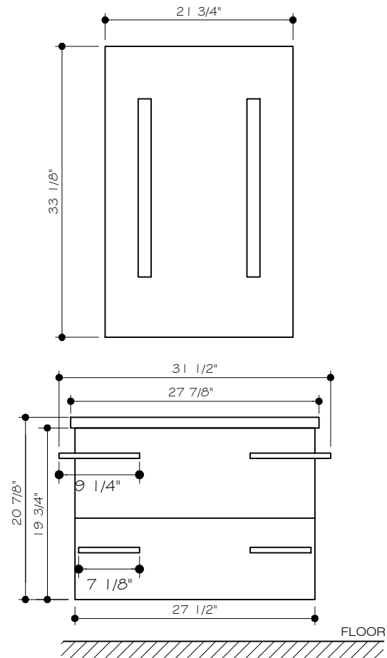
FRONT VIEW
