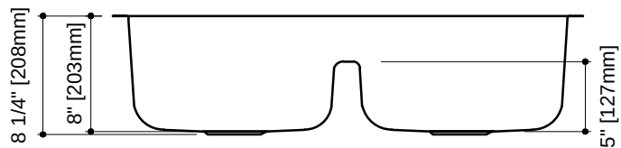
FRONT VIEW
